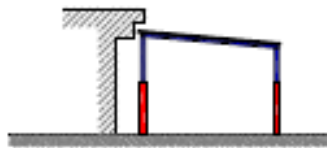
Proposed Arrangement of Early Years Fixed Canopy Structure – End View
