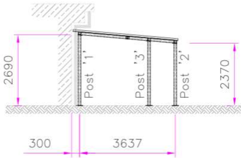
Details of 35m Long Fixed Canopy Structure – End
